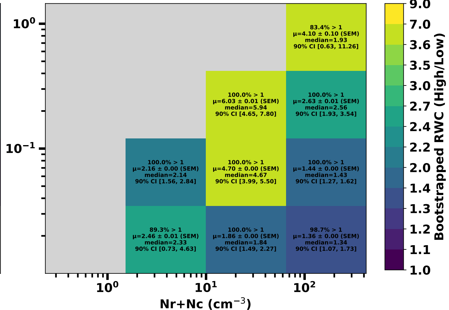
CDP RWC GCCN Concentration
